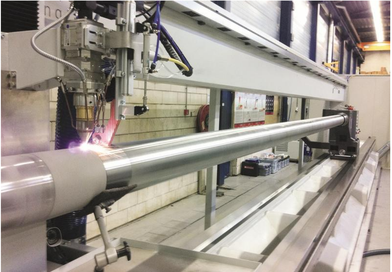
World premiere: EHLA system for Laser Material Deposition of piston rods having a length of up to ten meters. © Fraunhofer ILT, Aachen, Germany / Hornet Laser Cladding B.V., Lexmond, NL.
