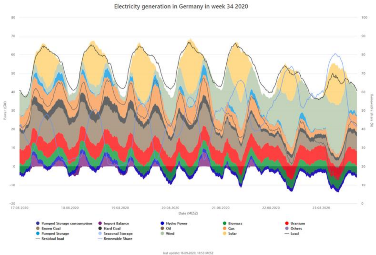
Graph showing electricity production in the 34th calendar week. Fraunhofer ISE; energy-charts.info
