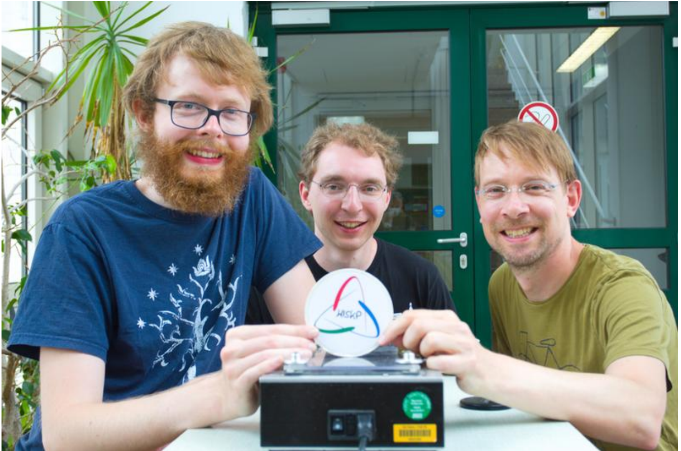
Investigating the trajectory of beer mats: the physics team Christoph Schürmann, Johann Ostmeyer and Prof. Dr. Carsten Urbach (from left). uni-bonn.tv © Carsten Urbach
