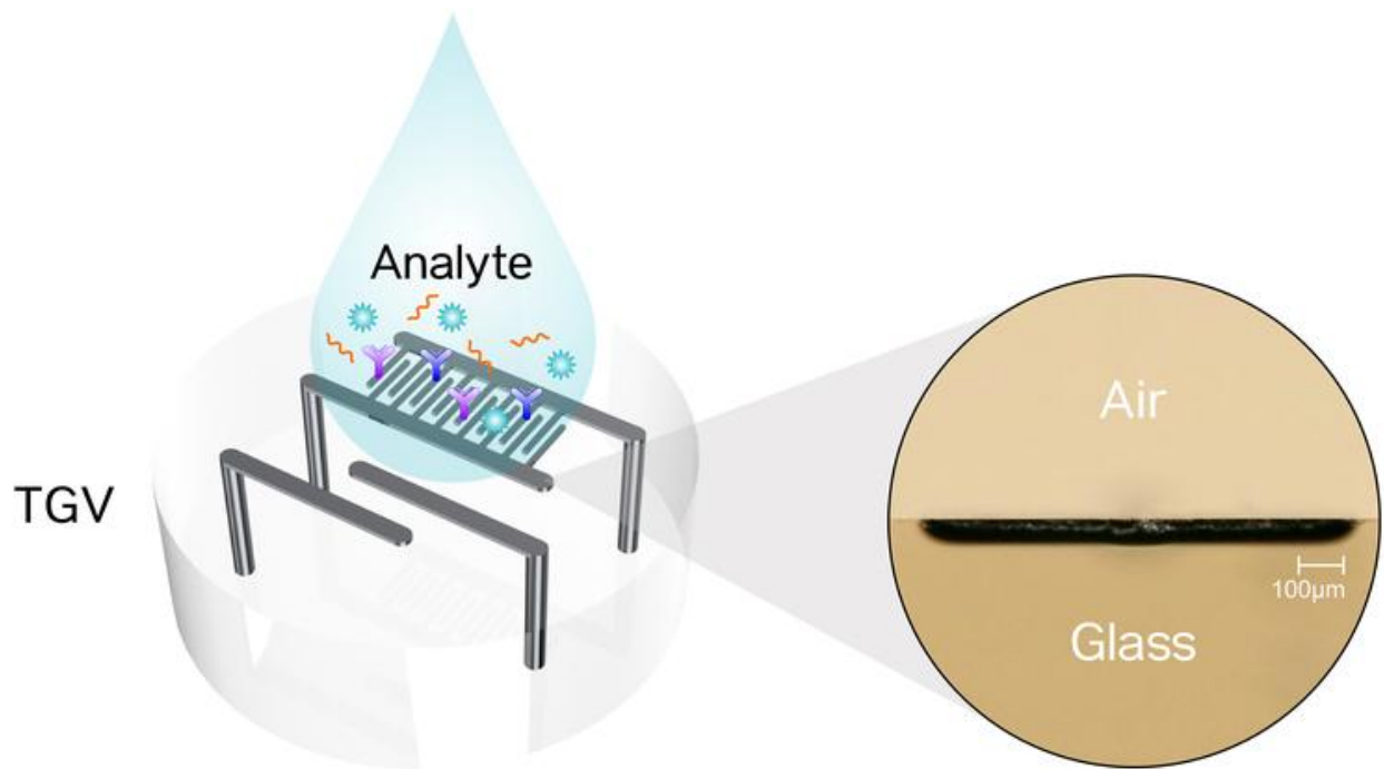
Proposed biosensor with glass-integrated metal structures to detect enzyme reactions or antigen antibody interactions. © Fraunhofer IZM
