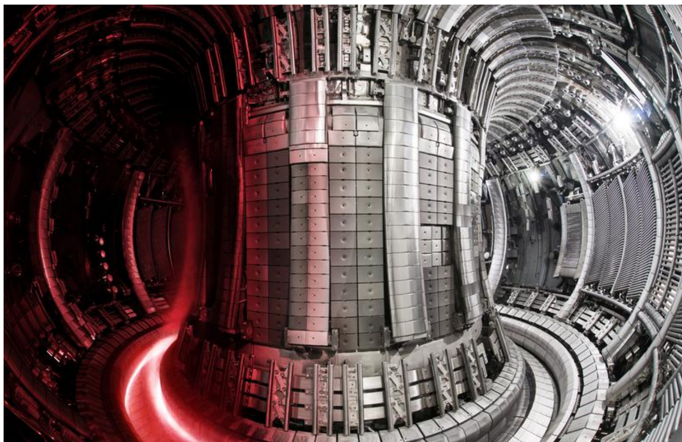
JET interior with superimposed plasma
