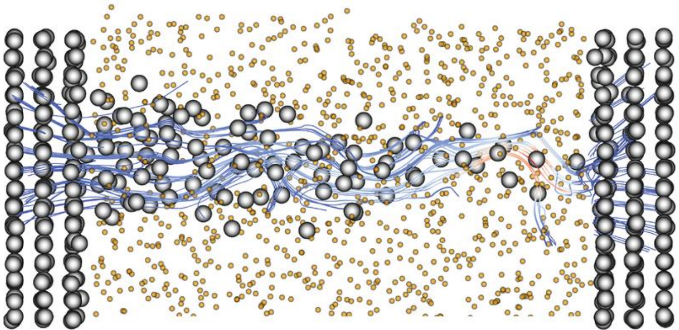
Atomic-scale computer simulation of a CBRAM cell subjected to 1mV voltage: electron trajectories (blue and red lines); copper atoms (grey); silicon and oxygen atoms (orange). © Mathieu Luisier / ETH Zurich
