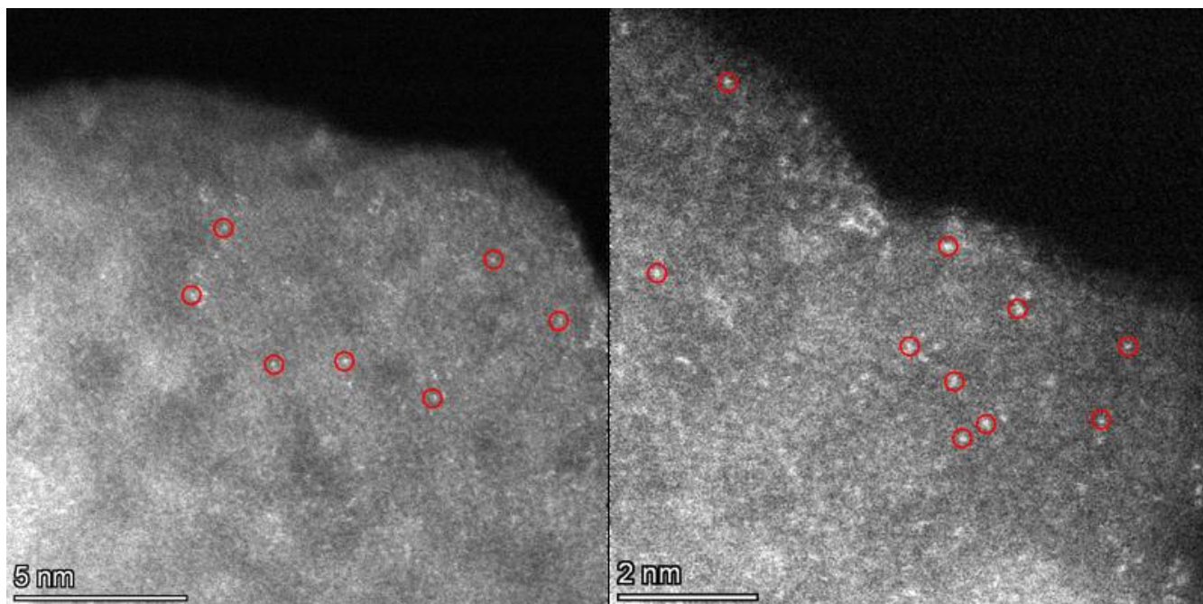
High-resolution image of the individual copper atoms (marked in red) of the heterogeneous catalyst (Cu-SAC) using a scanning transmission electron microscope (STEM). LIKAT
