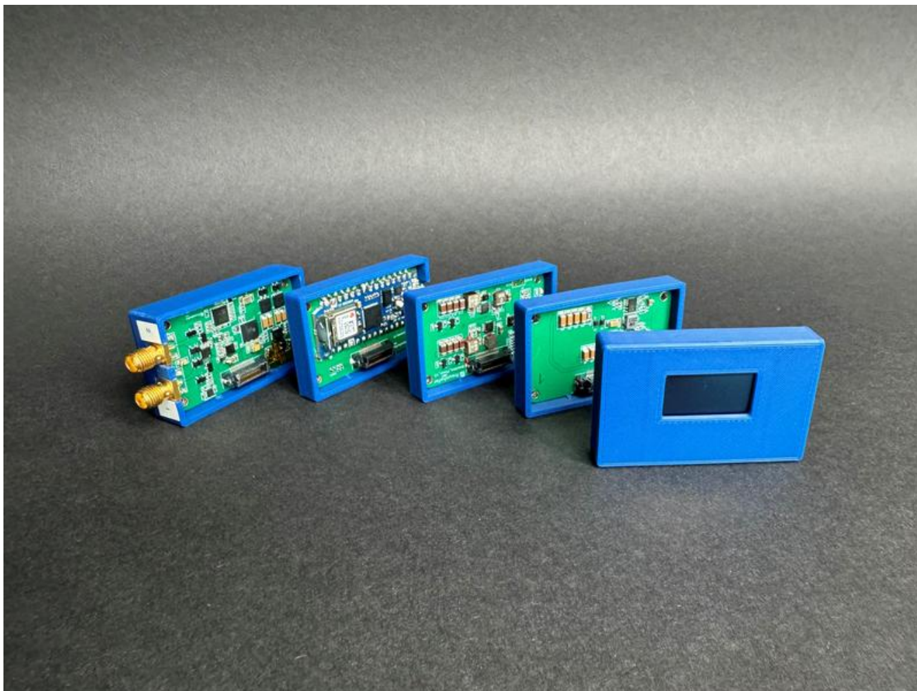
Individual modules of the “SonoOne” ultrasound system. Fraunhofer IBMT
