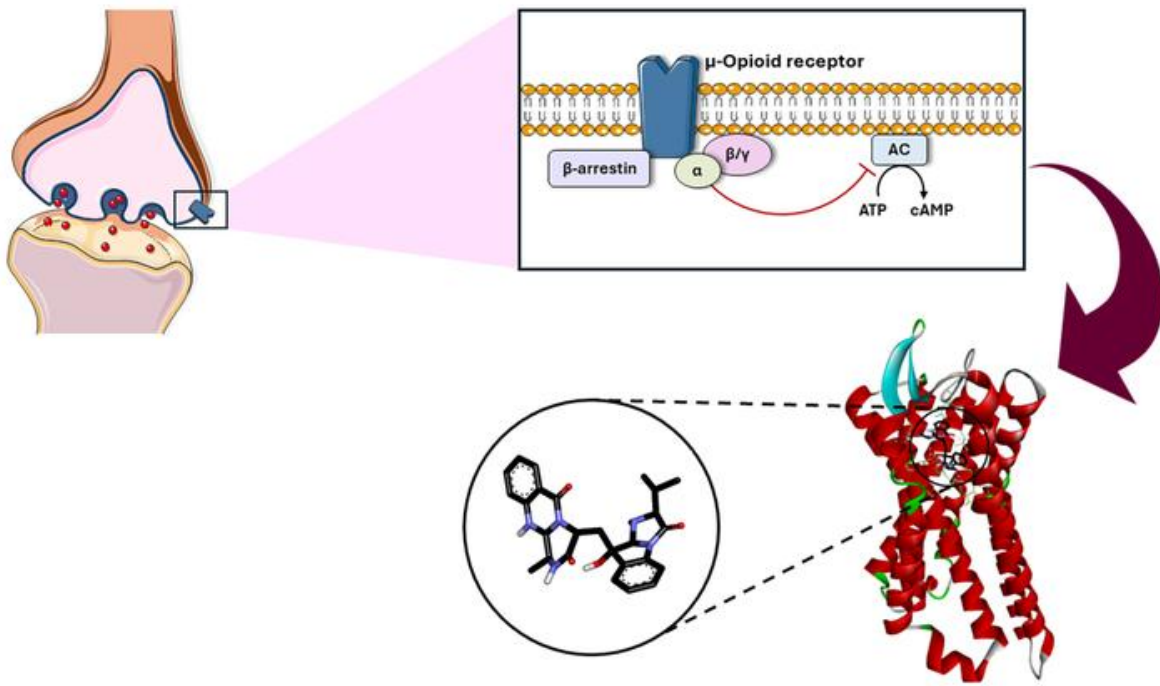
Binding of Aniquinazoline B to μ-opioid receptor
