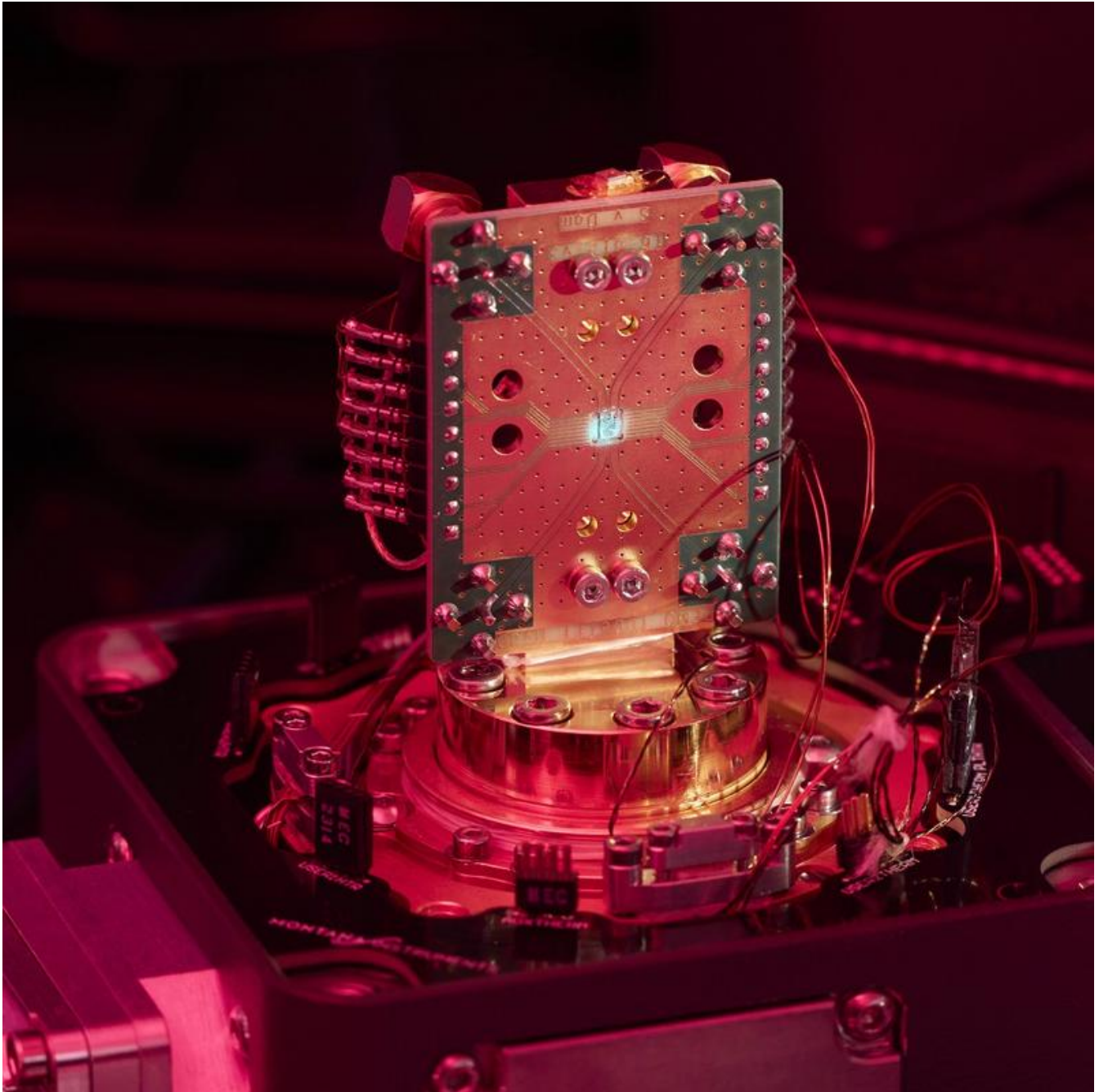
The heart of the quantum internet node is a cultured diamond with specifically introduced nitrogen vacancies (NV centers). It emits single photons that can carry and transport information about the state of the qubit. © Fraunhofer ILT, Aachen, Germany / Ralf Baumgarten.
